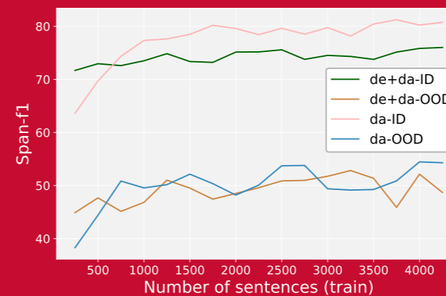
Figure 2: Learning curve for multi-task, mlBERT on in-domain (ID) news and average over all out-of-domain datasets (OOD).
