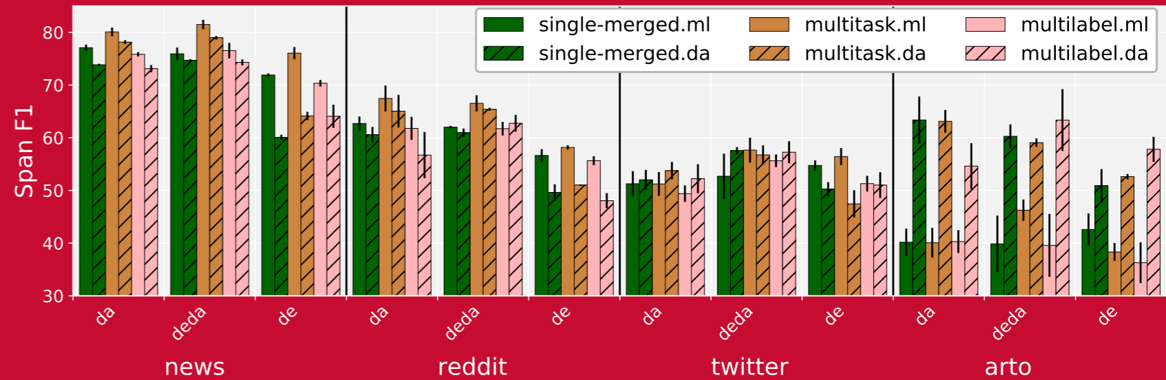
Figure 1: Nested NER results. Models trained on German (de), Danish (da) or both (de+da) and with mlBERT (ml) vs danishBERT (da). Average over 3 runs. Std. dev. indicated as error line.
